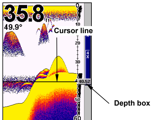
Sonar chart with the depth cursor active. The line indicates the large fish is 40.52 feet deep.
