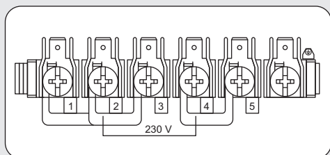
Bornier
