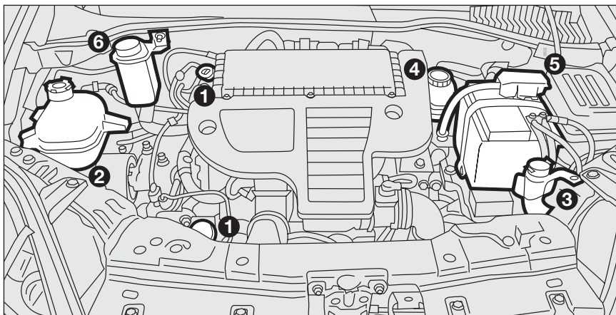
fig. 2 - Version 1.3 Multijet
