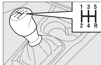
fig. 3 - Version 1.3 Multijet
