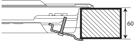
Plan 60 mm
