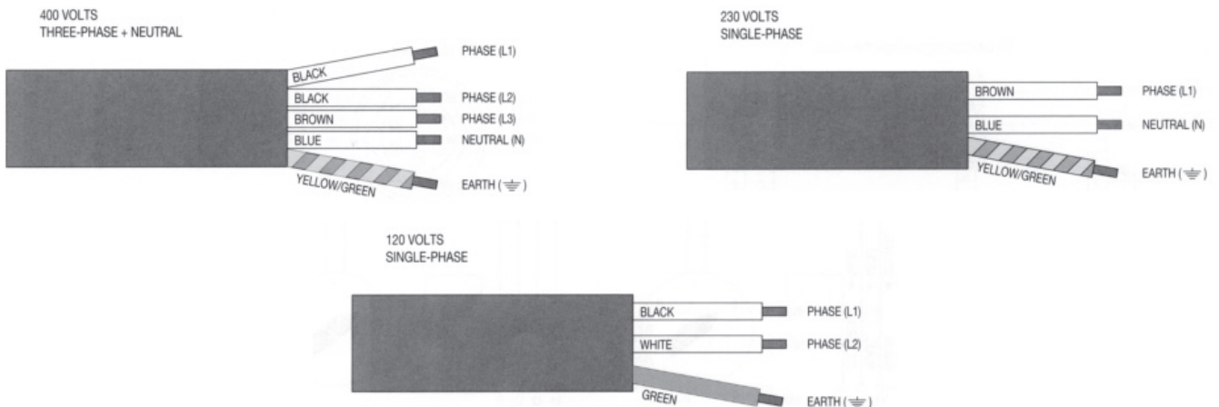
Feeding cable installation diagram
